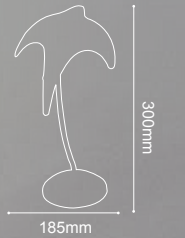
LD05-5427/1T Birds G9 MAX 40W x 1
