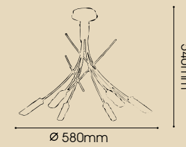
LC05-5420/6CB Mish mash G9 MAX 40W x 6
