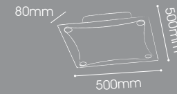
LD06-1500/4+1109 Plano G24 MAX 18W x 4
