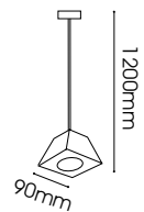
LT06-2209/02.2.1 Iceberg G9 MAX 40W x 1
