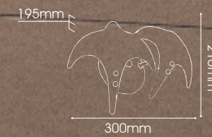
LD05-5427/2W Birds G9 MAX 40W x 2
